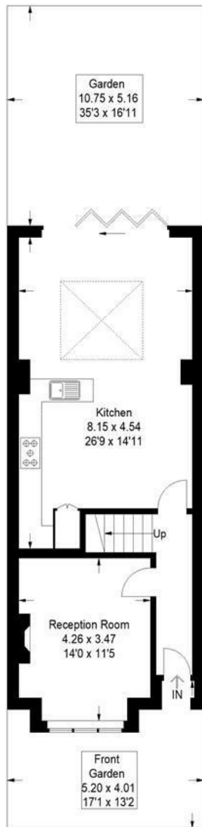
Ground Floor 605 sq ft / 56.2 sq m
